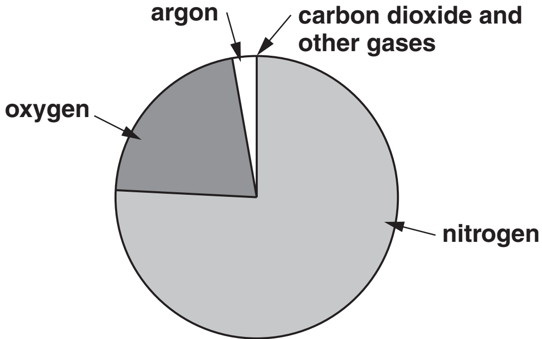
Fig. 1 Chemical composition of the Earth's atmosphere today
