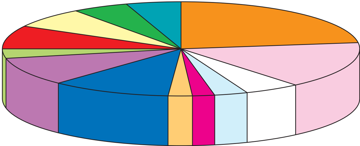
Fig. 1 Types of vegetation along a transect by %
