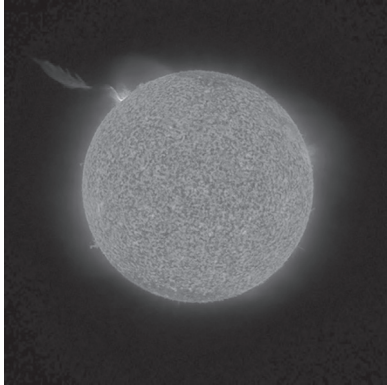
Fig. 4 A very large solar flare observed in 2017.
