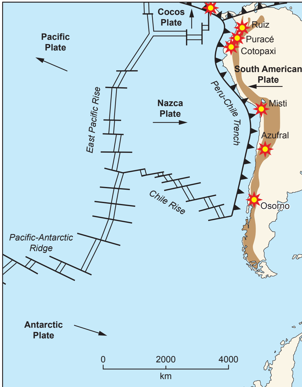
Fig. 5 – Plates and plate boundaries in the southeast Pacific
