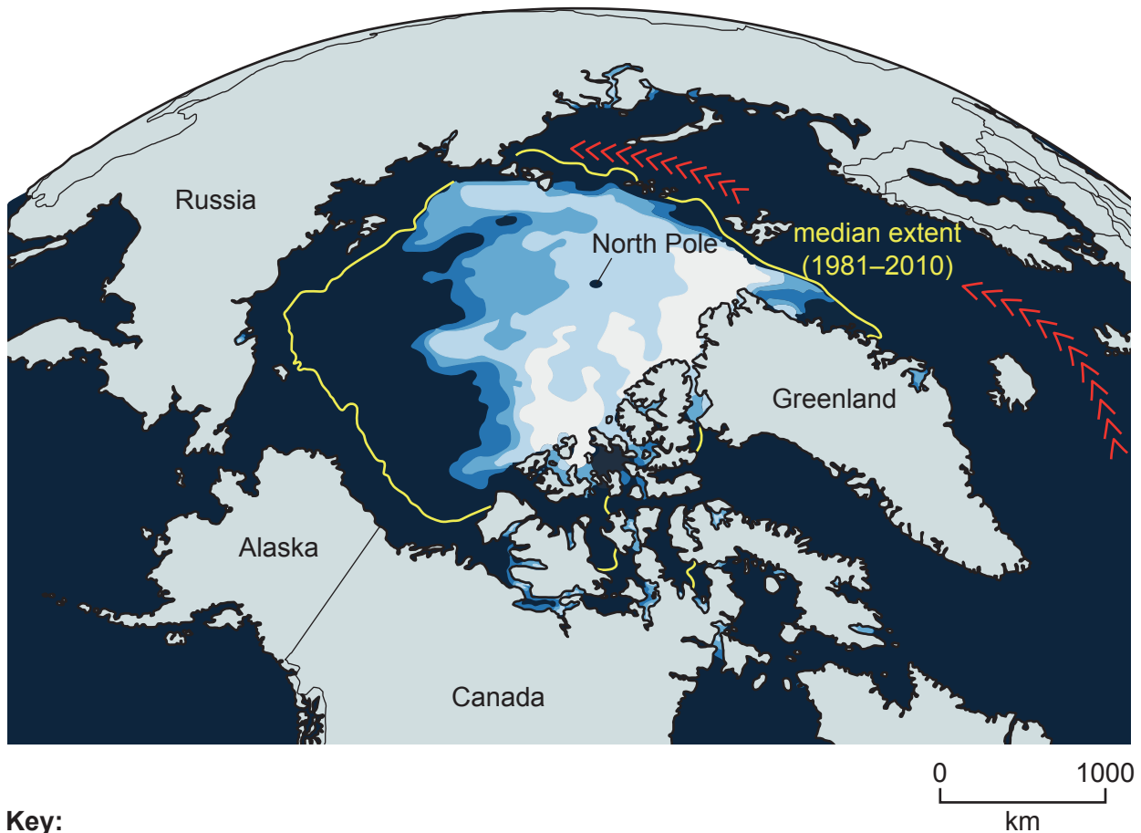
Fig. 1 – Decreasing extent of Arctic sea ice
