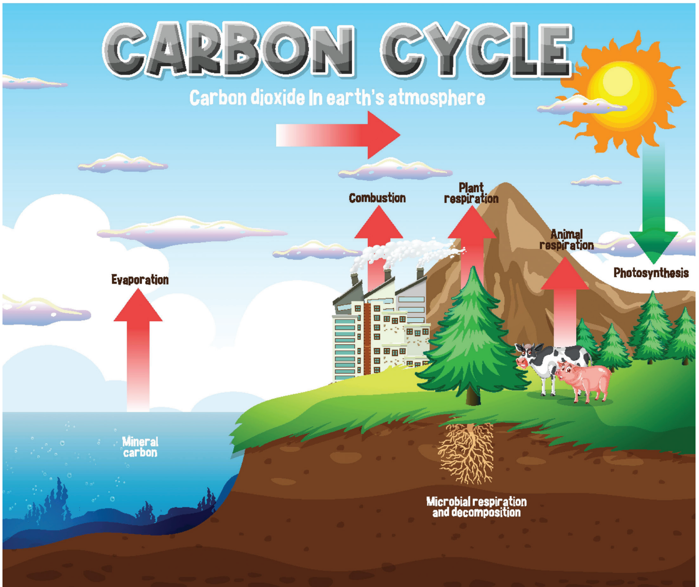
Fig. 6 – The Carbon Cycle
